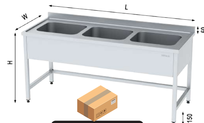
3 EVYELİ TEZGAH ALT TABLASIZ SINK WITH 3 BOWLS WITHOUT BOTTOM SHELF
