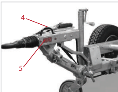
4 - Electrical Connection Socket 5 - Safety break arm
