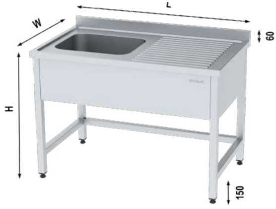
TEK EVYELİ ÇALIŞMA TEZGAHI ALT TABLASIZ WORK TABLE WITH SINGLE SINK WITHOUT BOTTOM SHELF
